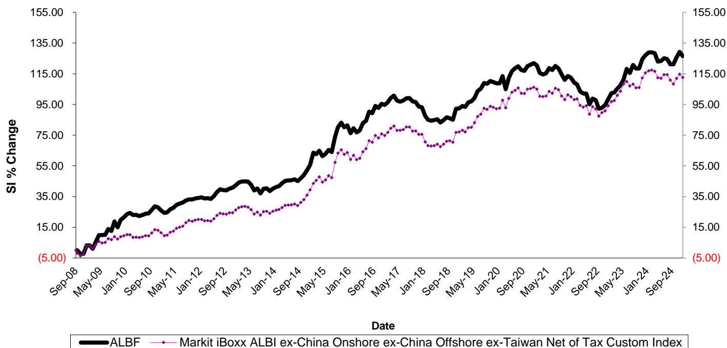
PRULink Asia Local Bond Fund Vs. Markit iBoxx ALBI ex-China Onshore ex-China Offshore ex-Taiwan Net of Tax Custom Index
