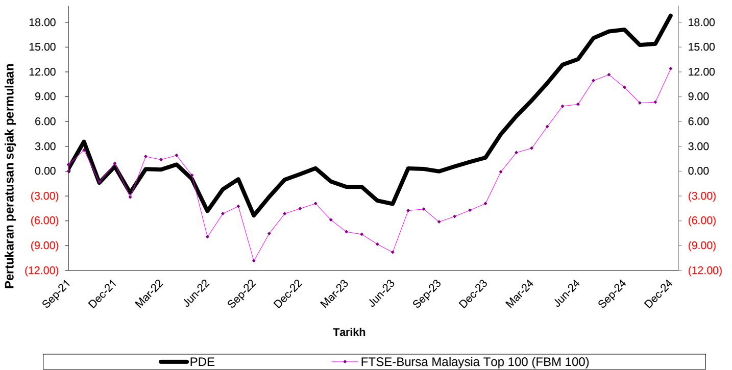
PRULink Dynamic Equity Fund Vs. FTSE-Bursa Malaysia Top 100 (FBM 100)
